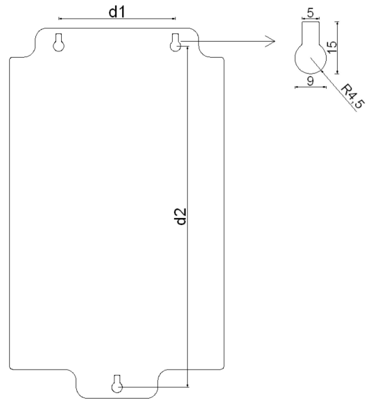
Figure 2.2 Mounting Holes
