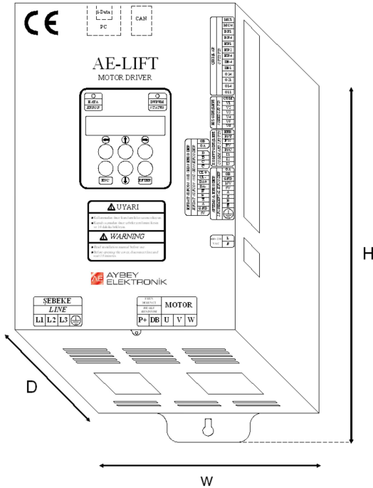
Figure 2.1 Device Box
